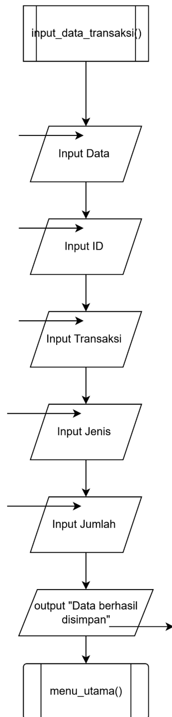
1.3 Flowchart tambah transaksi (create)
